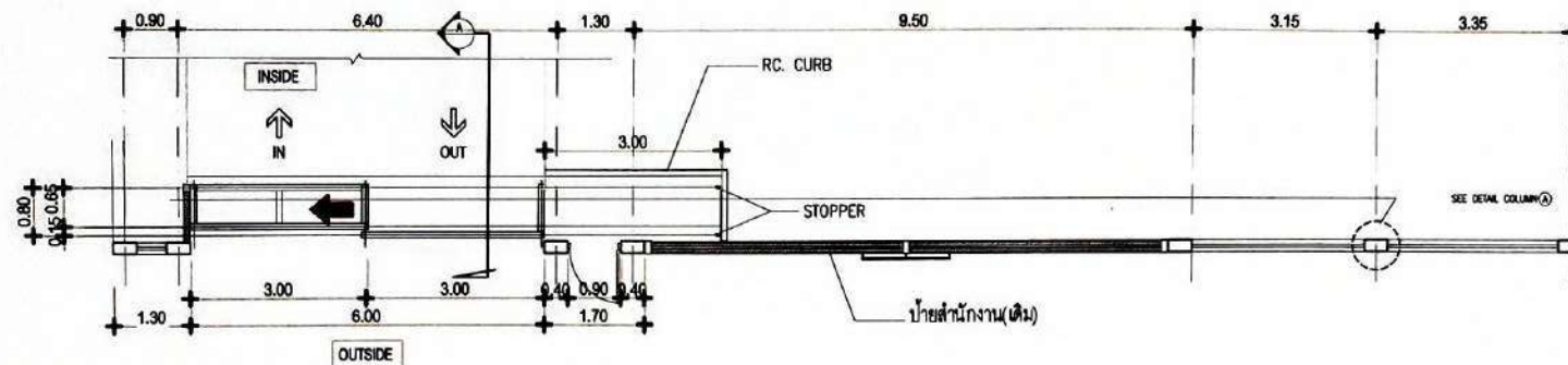
PLAN MAIN GATE SCALE 1:100
