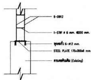
DETAIL COLUMN A SCALE 1:25
