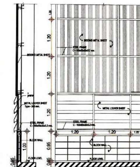
SECTION SCALE 1:50 INSIDE ELEVATION SCALE 1:50
