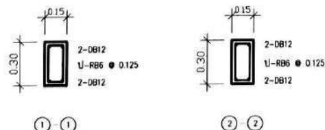
B8 Scale 1 : 25
