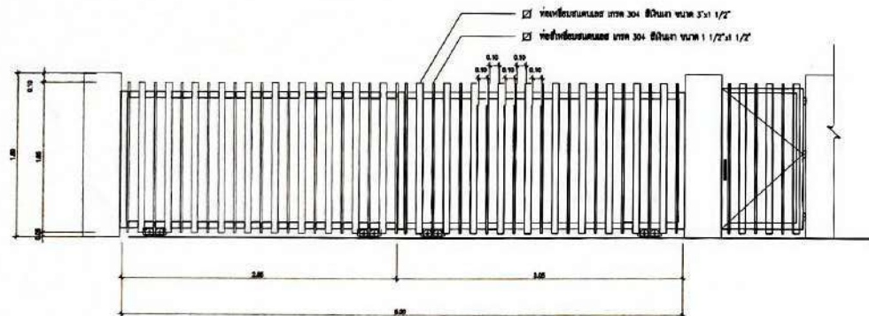
ELEVATION MAIN GATE SCALE 1:10
