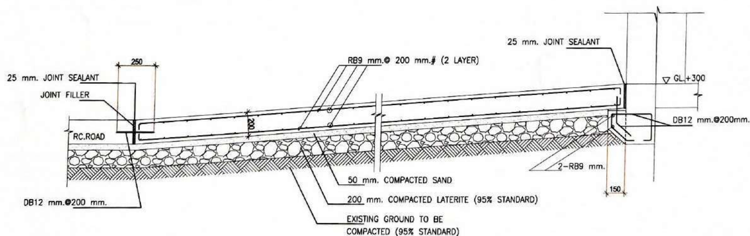
RC. RAMP DETAIL
