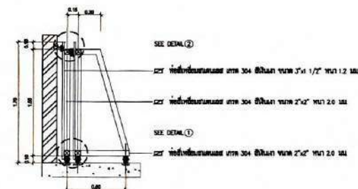
SECTION A SCALE 1:10
