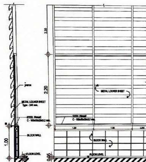
SECTION SCALE 1:50 INSIDE ELEVATION SCALE 1:50
