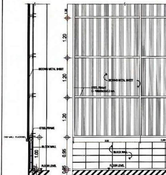
SECTION SCALE 1:50 INSIDE ELEVATION SCALE 1:50
