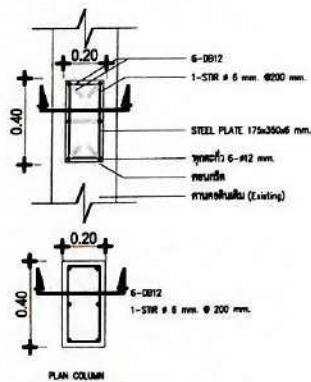
PLAN COLUMN
