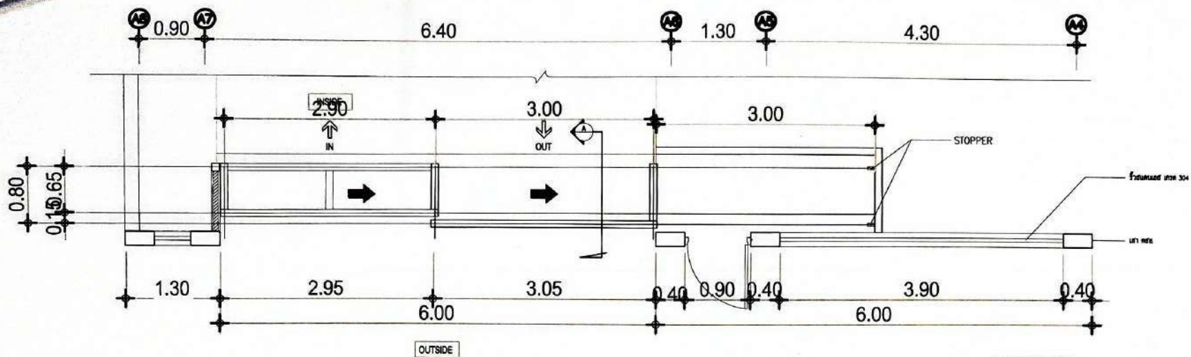
PLAN MAIN GATE SCALE 1:10
